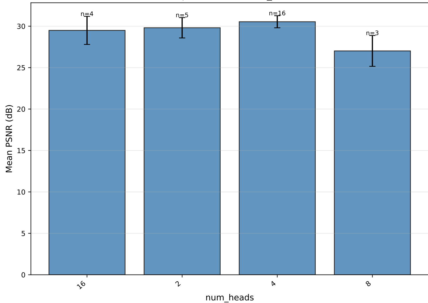
Mean PSNR per value of num_heads — HAT
